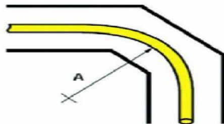
Minimum bend radius - 15 x pipe outside diameter
